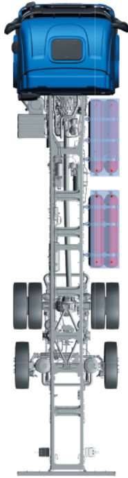
CNG tanks on the right side, available in combination with, on the left side: • LNG • CNG • Free
