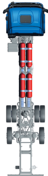
CNG tanks on the chassis, available in combination with: • Right side CNG; left side free • Right side free, left side CNG
